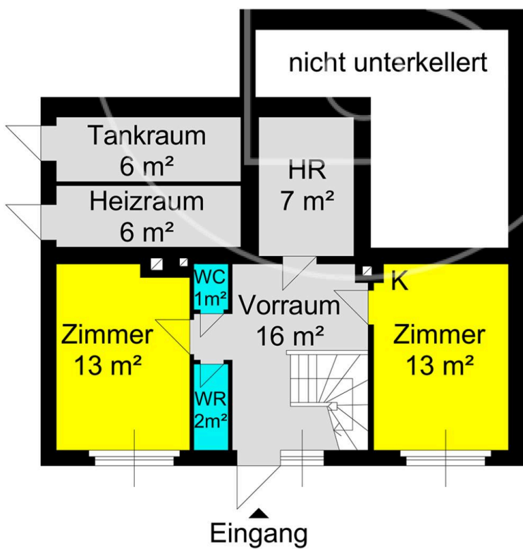
K ... Kamin HR ... Heizraum WR ... Waschraum Skizze Erdgeschoss
